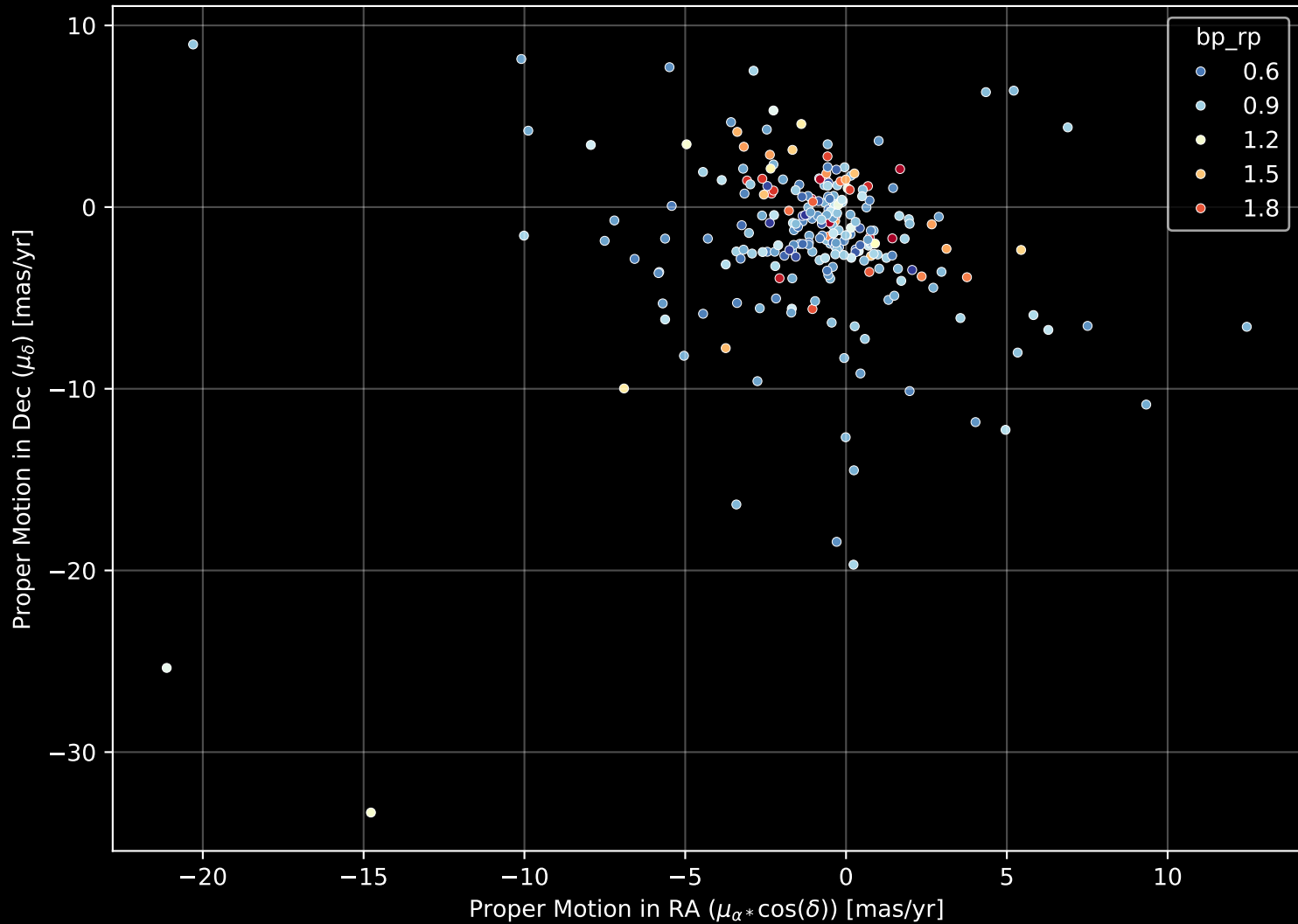
GALAH DR4 Field: [9222] Proper Motion Diagram (n= 245)
