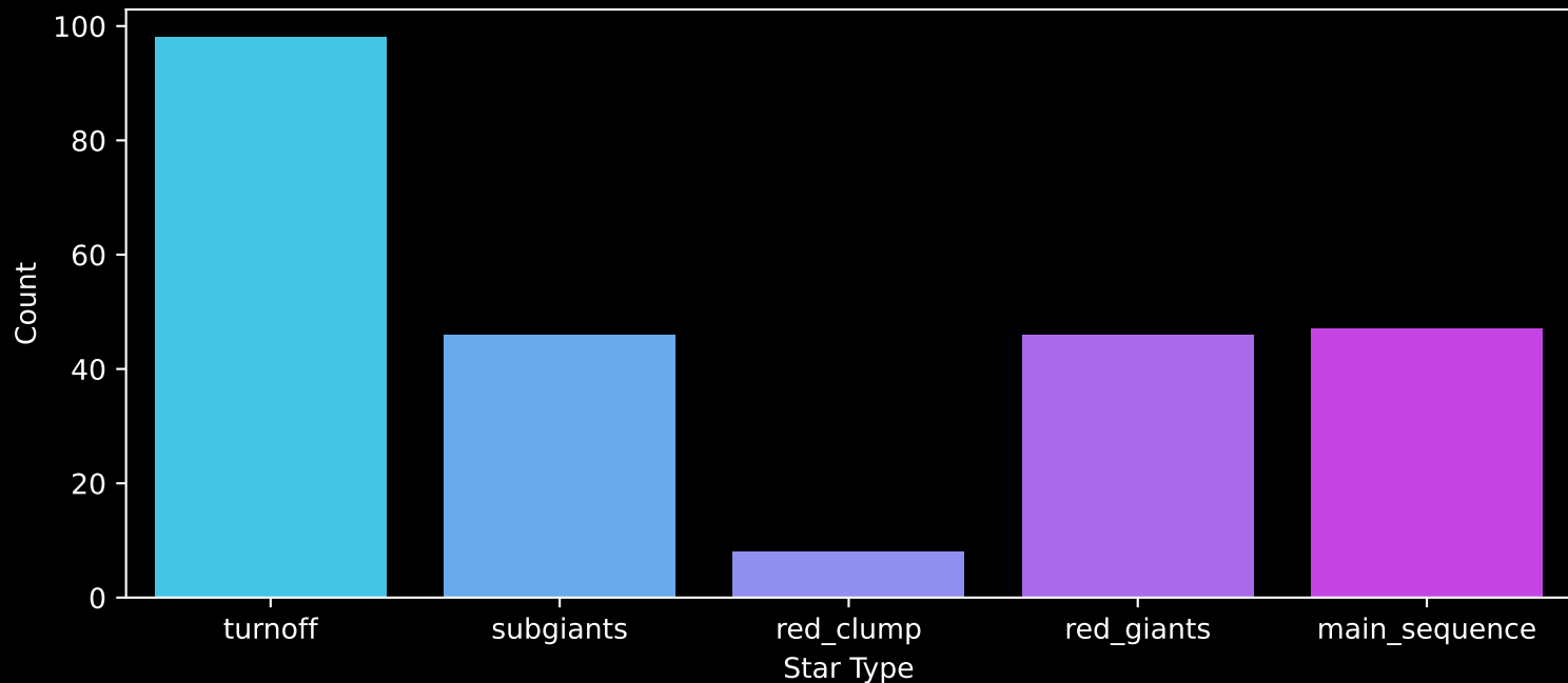
GALAH DR4 Field: [9222] Count plot of Star Type
