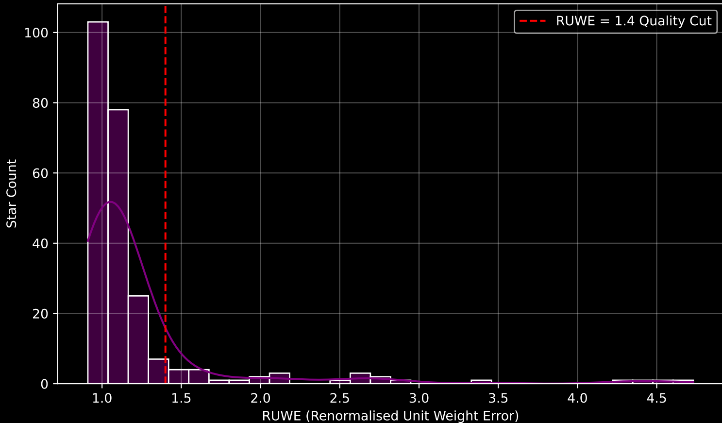
GALAH DR4 Field [9222] RUWE Distribution (n= 240)
